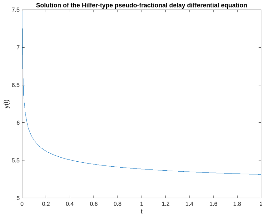
FIG. 1. Solution of the Eq. (7.1) within the interval [0, 2] .
